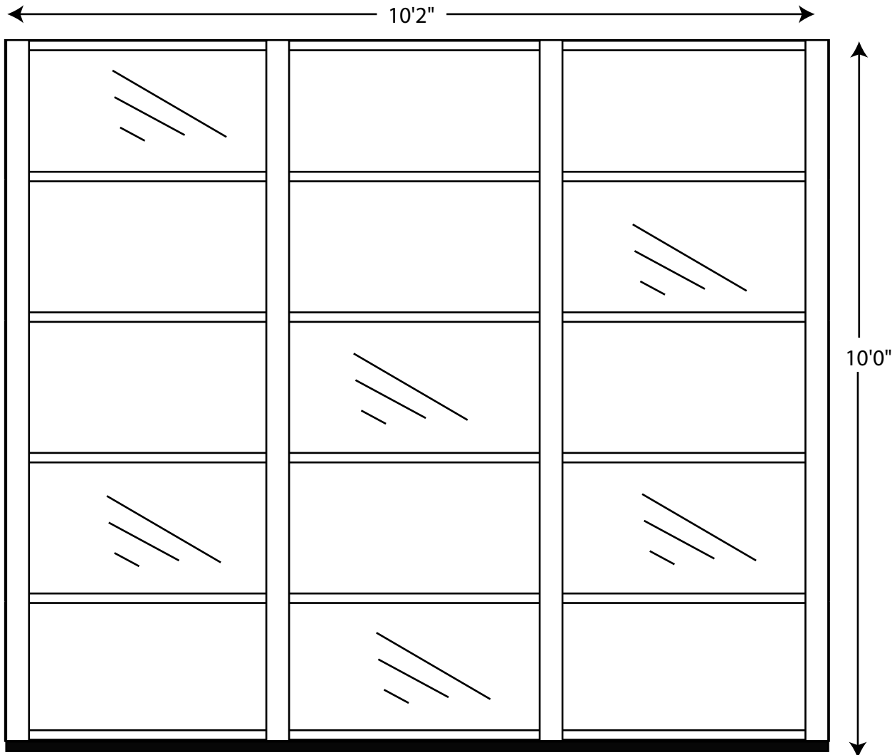
Full Vision Section Side Elevation
