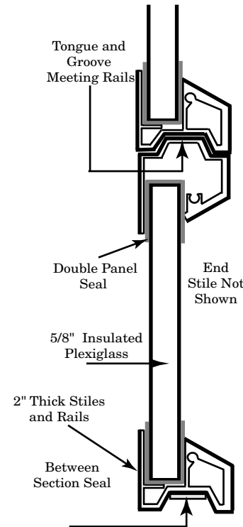
Full Vision Section Side Elevation
