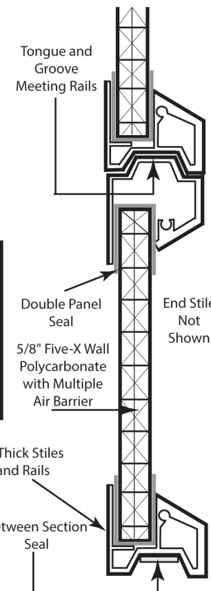
Polycarbonate Section Side Elevation
